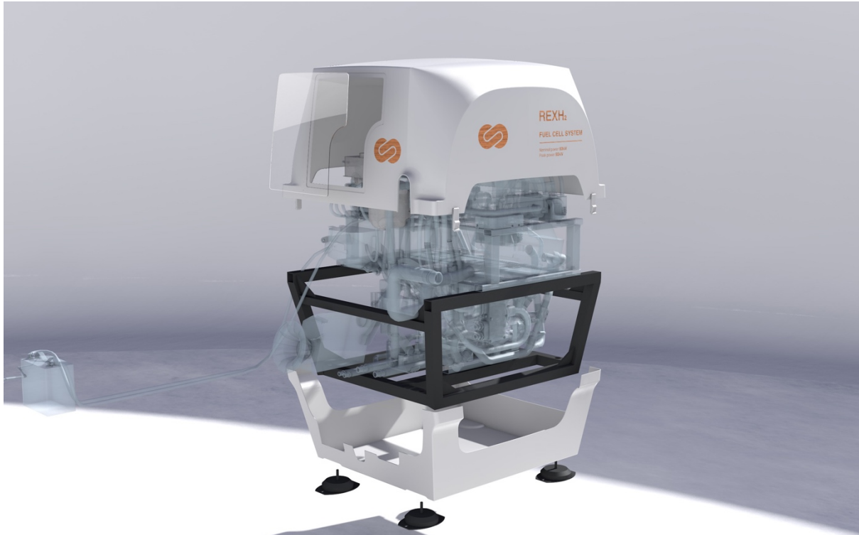
3D rendering REXH2 with its cover © EODev / Jean Hiss
